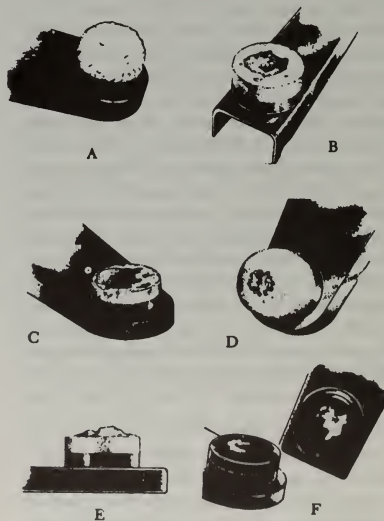
FIGURE 4-64. Examples of contact surface condition.
